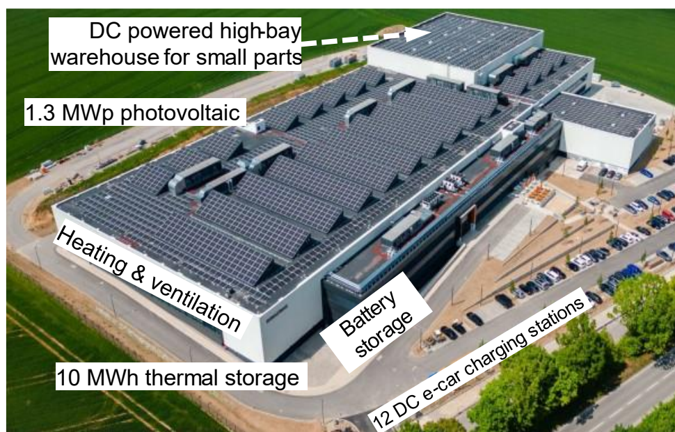
Figure 3 Aerial view of Schaltbau building [10]
